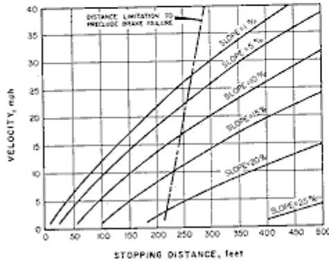
FIGURE 3. - Stopping distance characteristics of vehicles of 200,000 to 400,000 pounds GVW.
