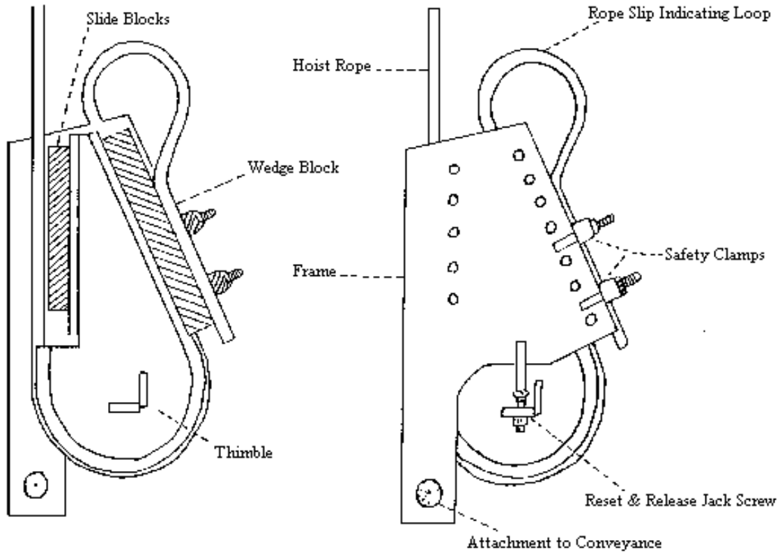
SHORT COUPLED THIMBLE
