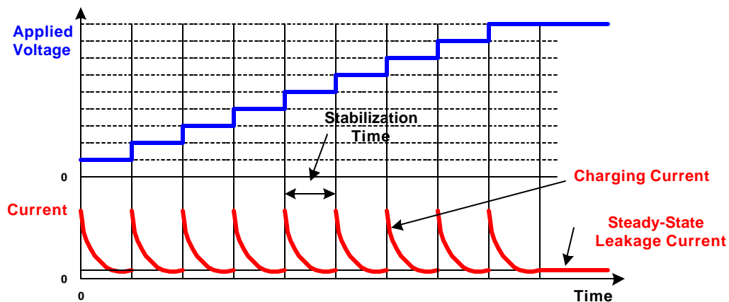
Figure 8: Charging Current
